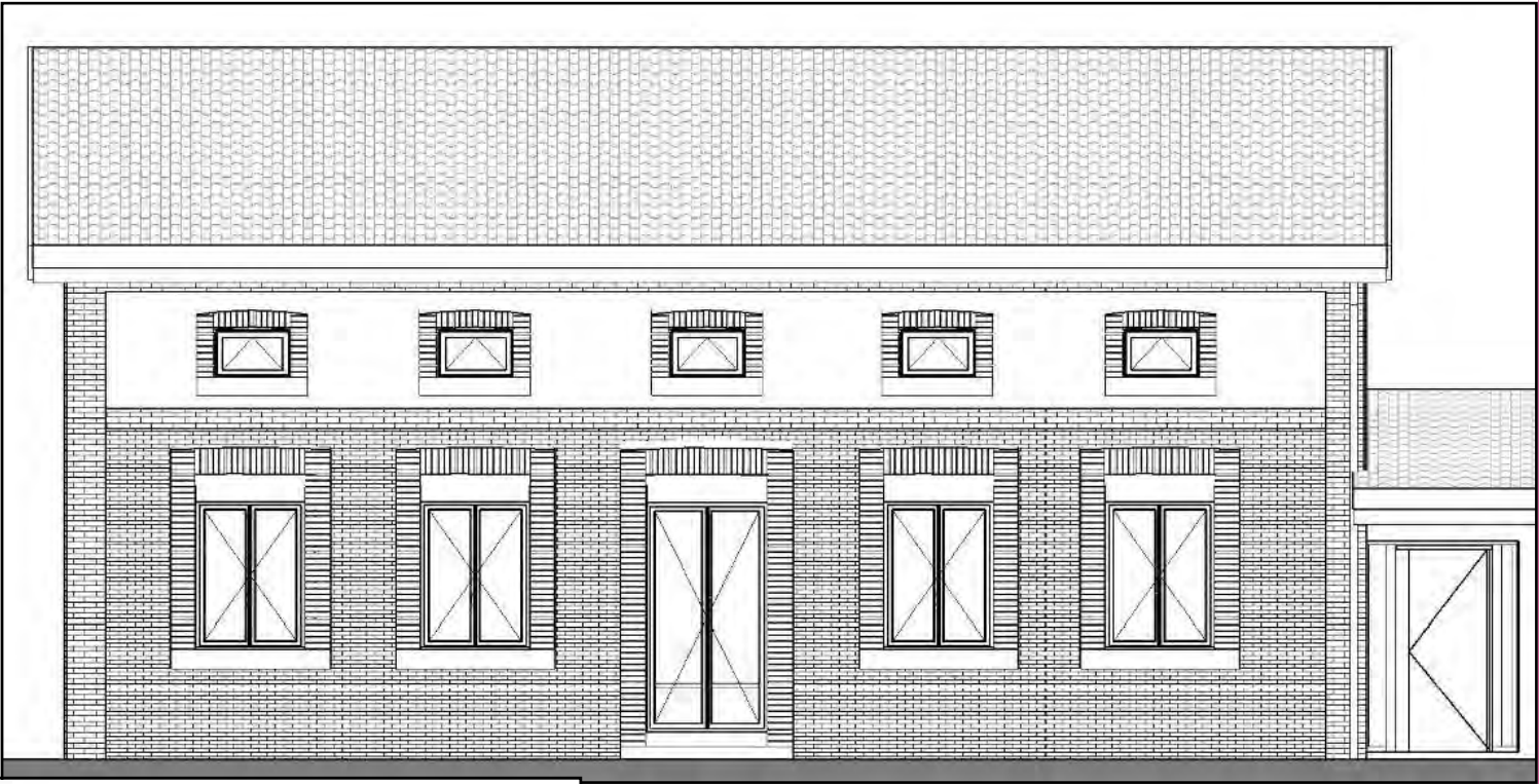
Façade principale
